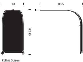
Rolling Screen
